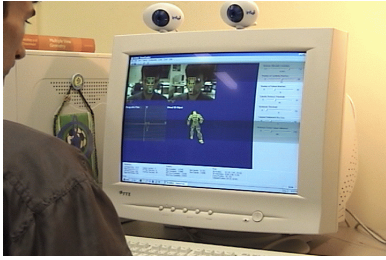
Figure 1: Stereo tracking with two web-cameras. The key issue is finding the relationship between the cameras.
